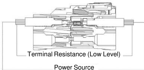
Figure 2: Low Level Contact Resistance Measuring Method (Resistance of the wire to be subtracted)
