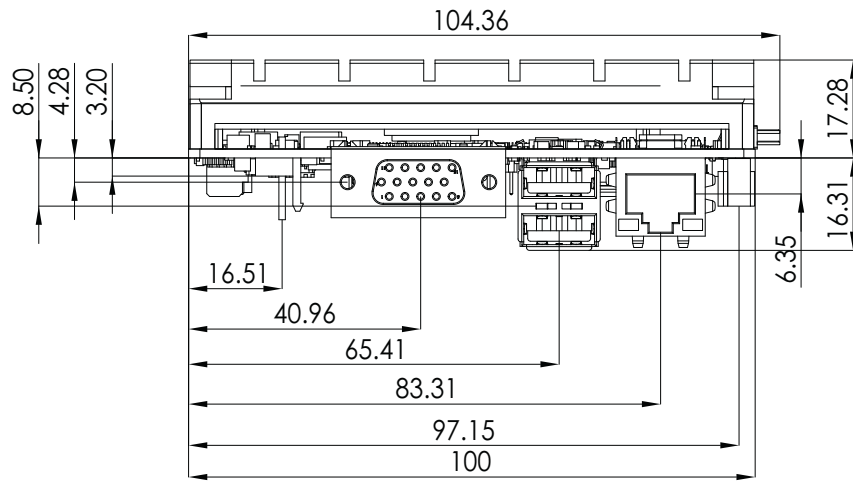
Figure 2.7 Board dimensions and layout (coastline with power connector and heat sink)
