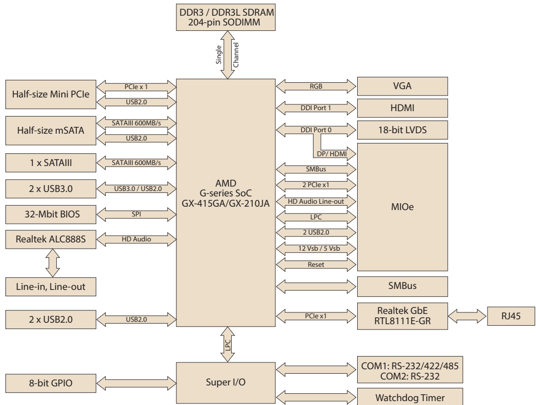
Figure 1.1 Block diagram
