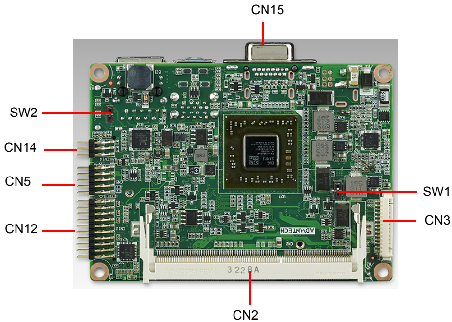
Figure 2.1 Jumper and connector layout (top side)
