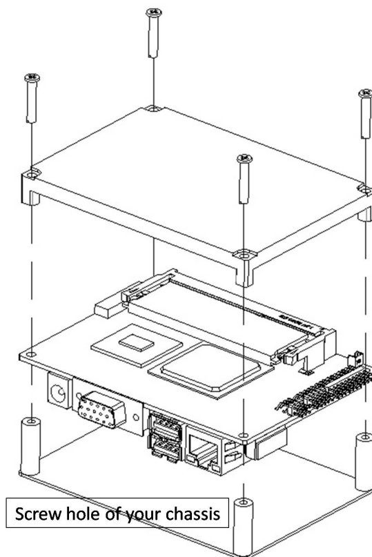
Figure 2.11 Heat spreader assembly
