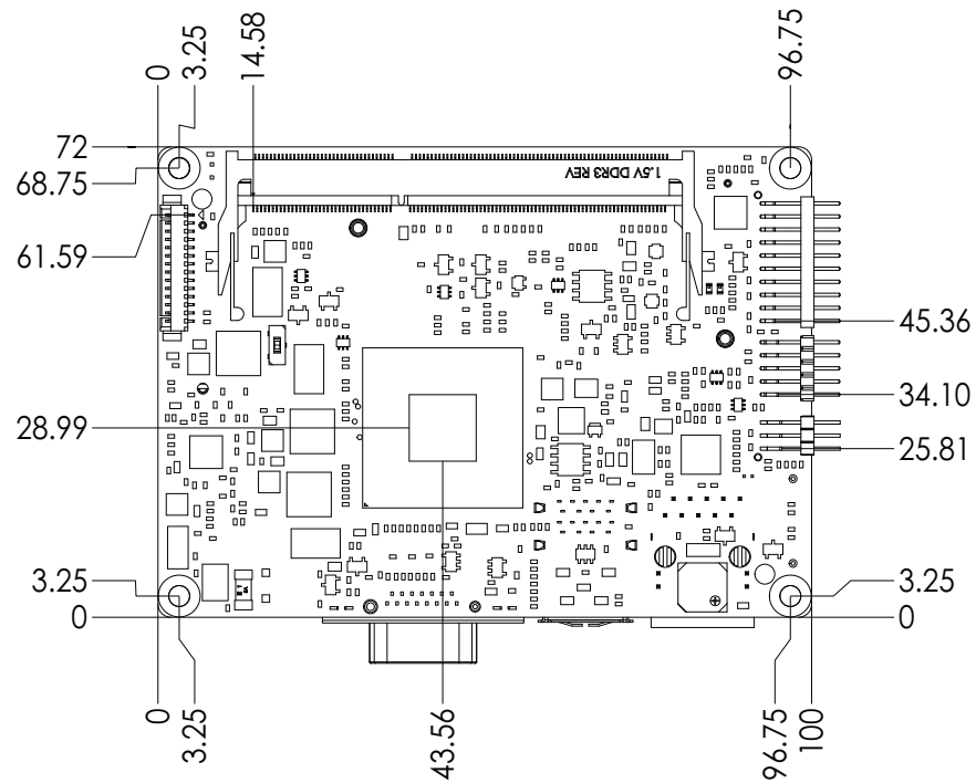
Figure 2.3 Board dimensions and layout (top side)
