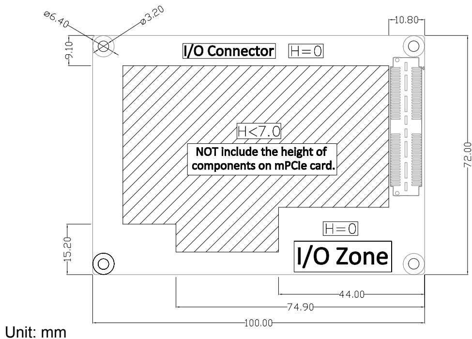
Figure 2.10 MI/O module height constraints
