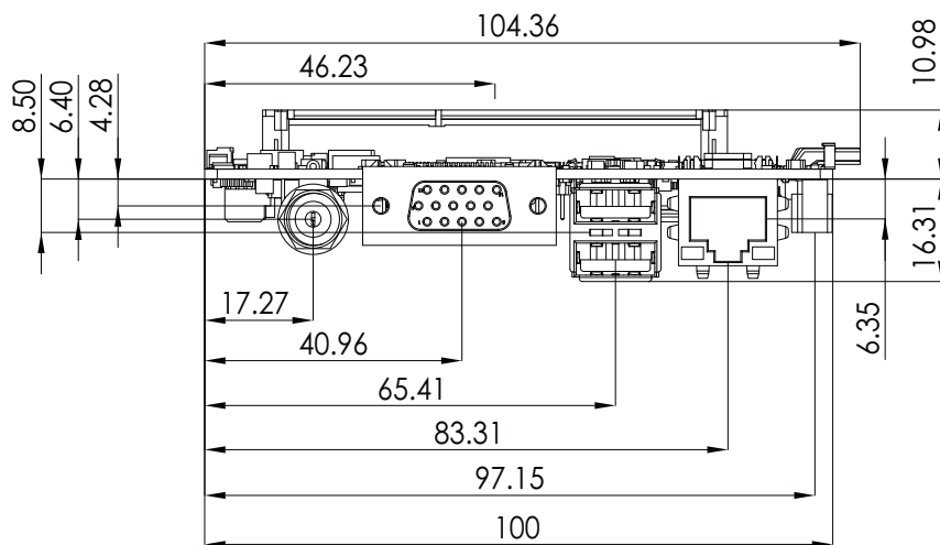
Figure 2.6 Board dimensions and layout (coastline with optional DC jack)
