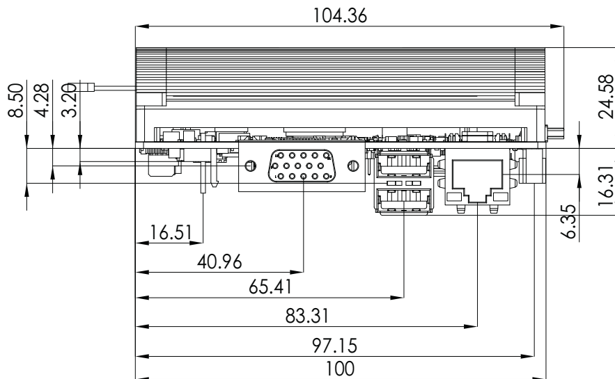
Figure 2.9 Board dimensions and layout (coastline with cooler)
