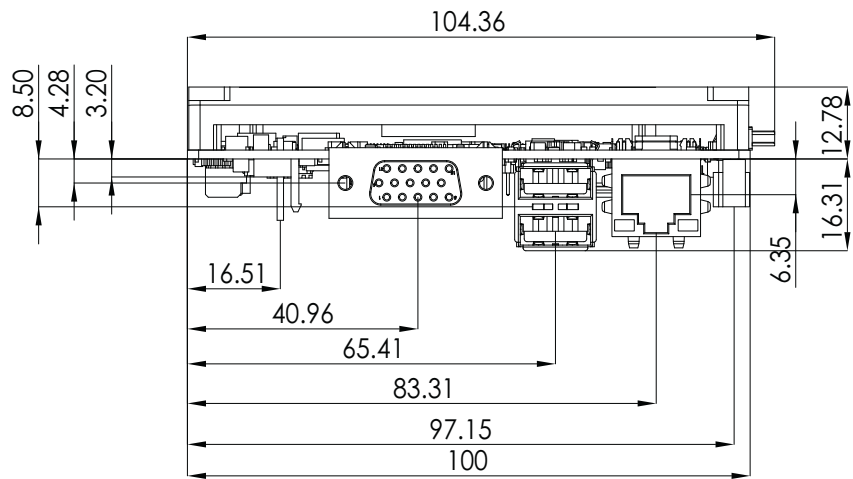
Figure 2.8 Board dimensions and layout (coastline with power connector and optional heat spreader)
