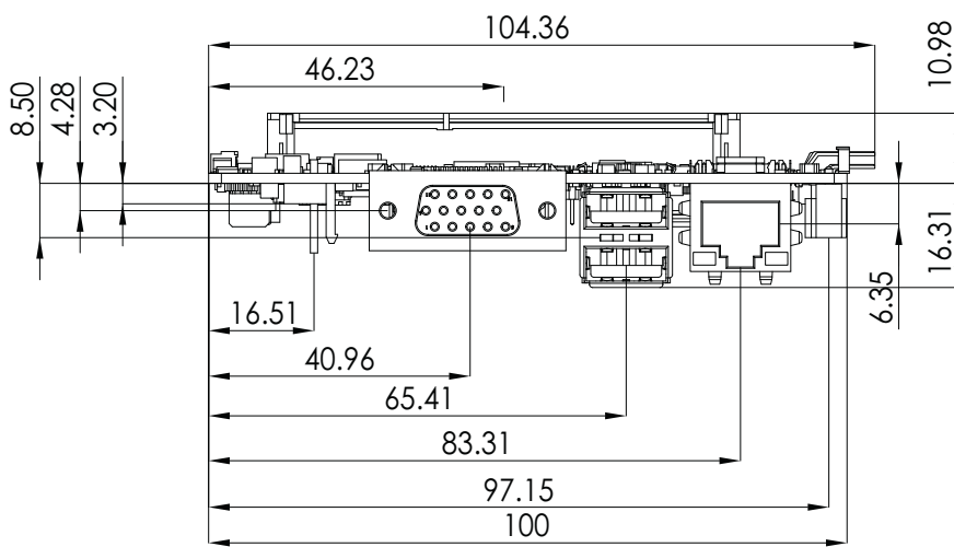
Figure 2.5 Board dimensions and layout (side view)
