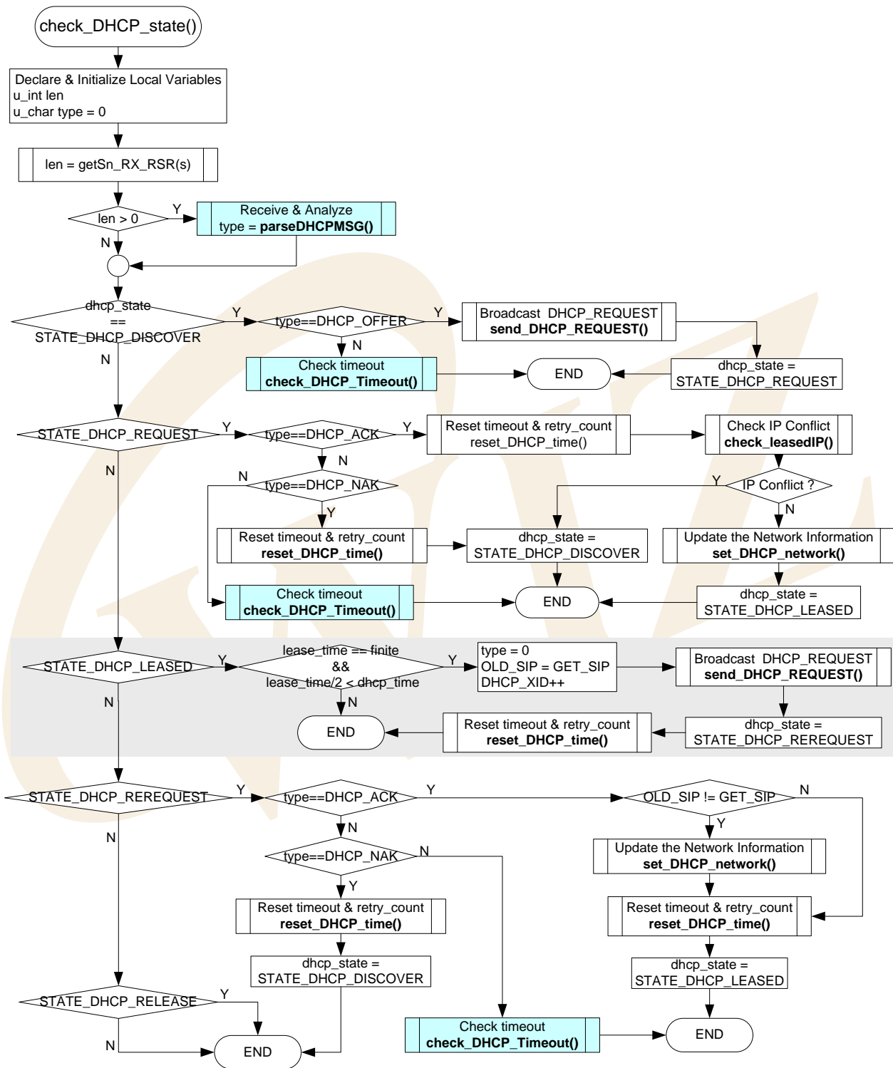
<Fig 3.31: check_DHCP_state()>
