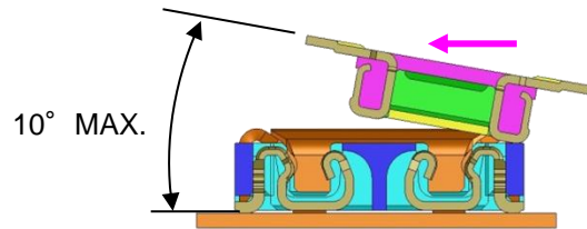
長手方向 "a" direction (lengthways)
