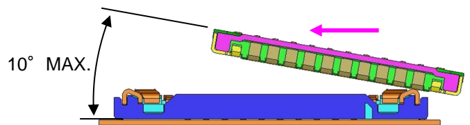
長手方向 "a" direction (lengthways)
