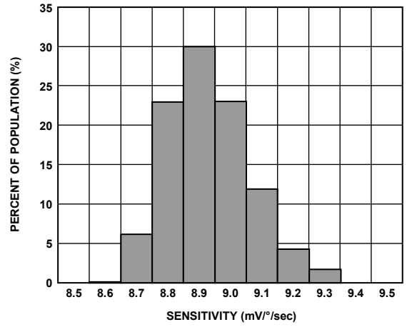
Figure 7. Sensitivity at 25°C
