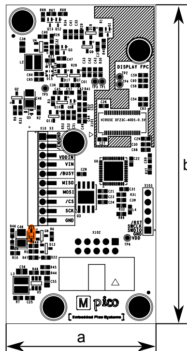
Figure 2.2: TCM2-P102 Outline
