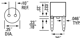
Circuit Board Mounting Detail
