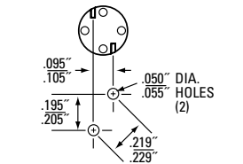
Circuit Board Mounting Detail
