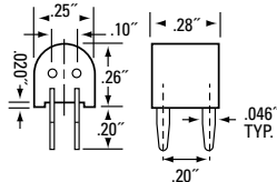
Circuit Board Mounting Detail
