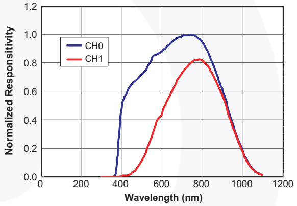
Fig. 4 Spectral Response
