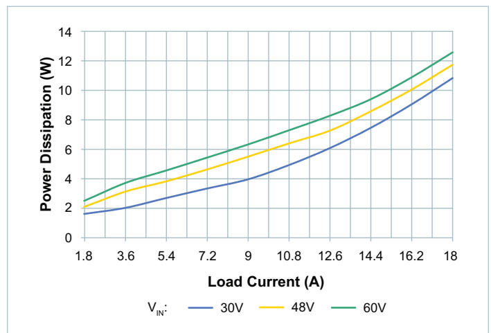
Figure 66 — System Power Dissipation, High Trim, Board Temperature = 100°C
