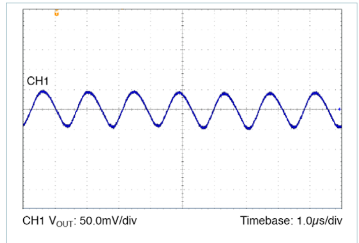
Figure 77 — Output Voltage Ripple: Nominal Line, Nominal Trim, 50% load, C OUT = 8 x 10µF Ceramic
