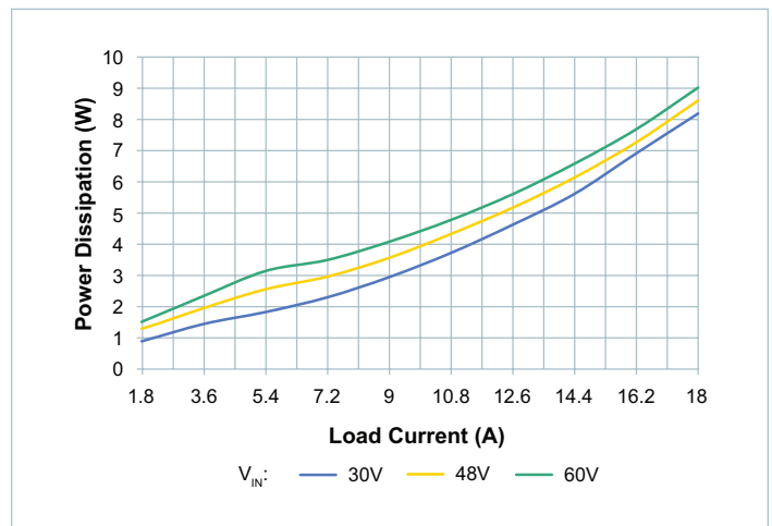
Figure 65 — System Power Dissipation, Low Trim, Board Temperature = 100°C
