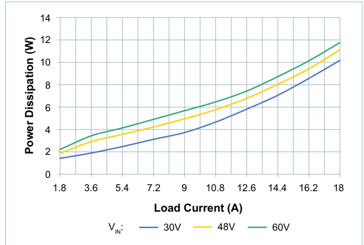
Figure 64 — System Power Dissipation, Nominal Trim, Board Temperature = 100°C
