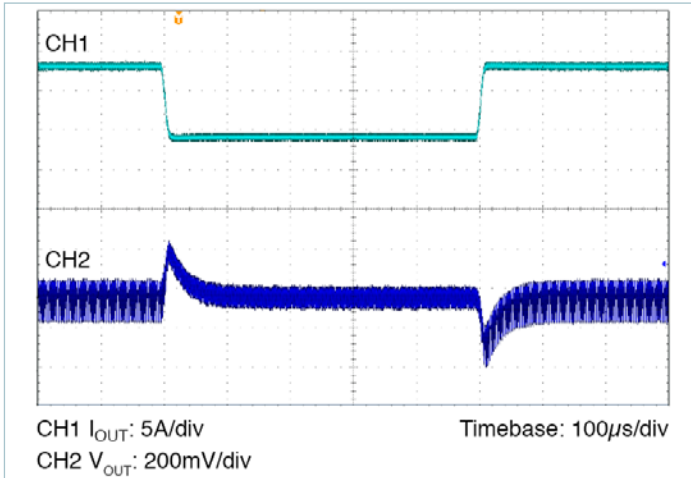
Figure 73 — Transient Response: 50% to 100% load, at 1A/µs. Nominal Line, Nominal Trim, C OUT = 8 x 10µF Ceramic
