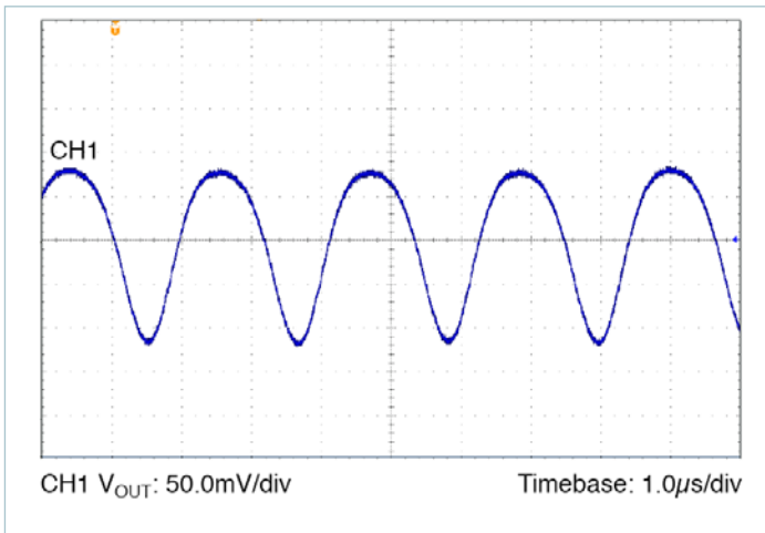
Figure 74 — Output Voltage Ripple: Nominal Line, Nominal Trim, 100% load, C OUT = 8 x 10µF Ceramic
