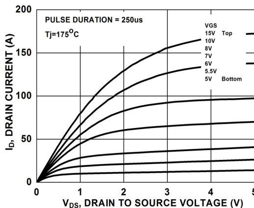
Figure 10. Saturation Characteristics
