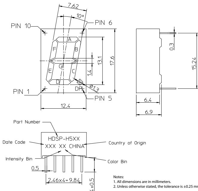
Figure 1 Package Dimension
