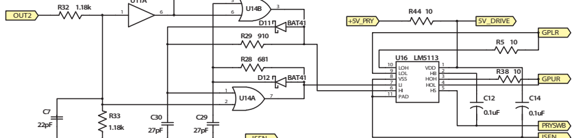
Primary Gate Drives
