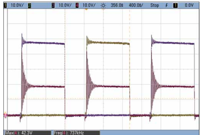
Figure 4: Typical waveforms taken at 48 V IN to 12 V OUT /15 A OUT CH1: Primary side switch node A voltage – CH3: Primary side switch node B voltage – CH4: Secondary side bridge voltage
