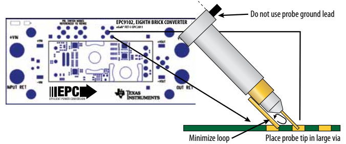
Figure 3: Proper Measurement of Switch Nodes or Output Voltage
