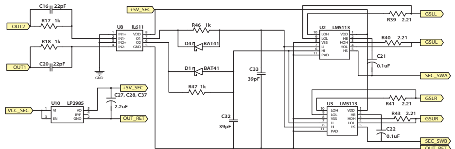
Secondary Gate Drives
