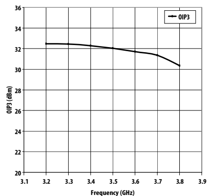
Figure 30. OIP3 vs Frequency
