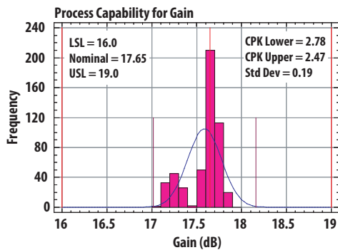
Figure 1. Gain distribution at 57mA
