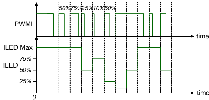
Figure 2. DC Dimming
