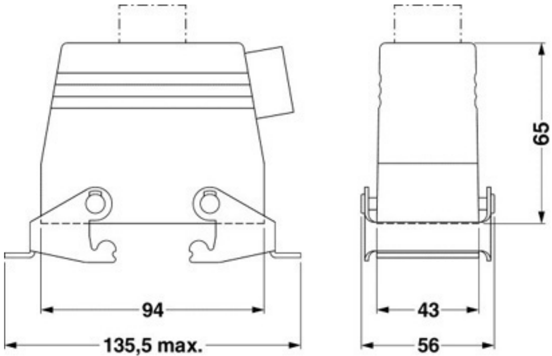
Dimensioned drawing
