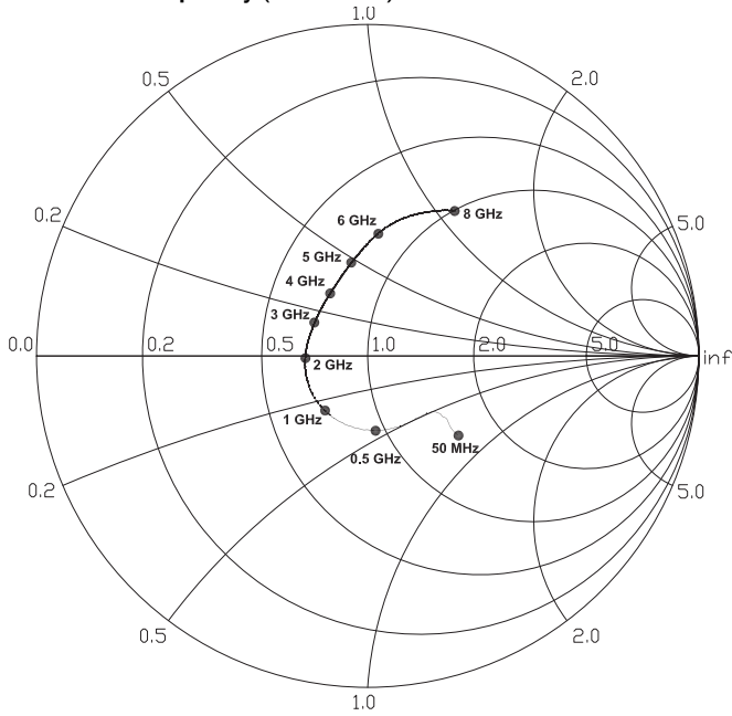
S11 versus Frequency (3V 25mA)
