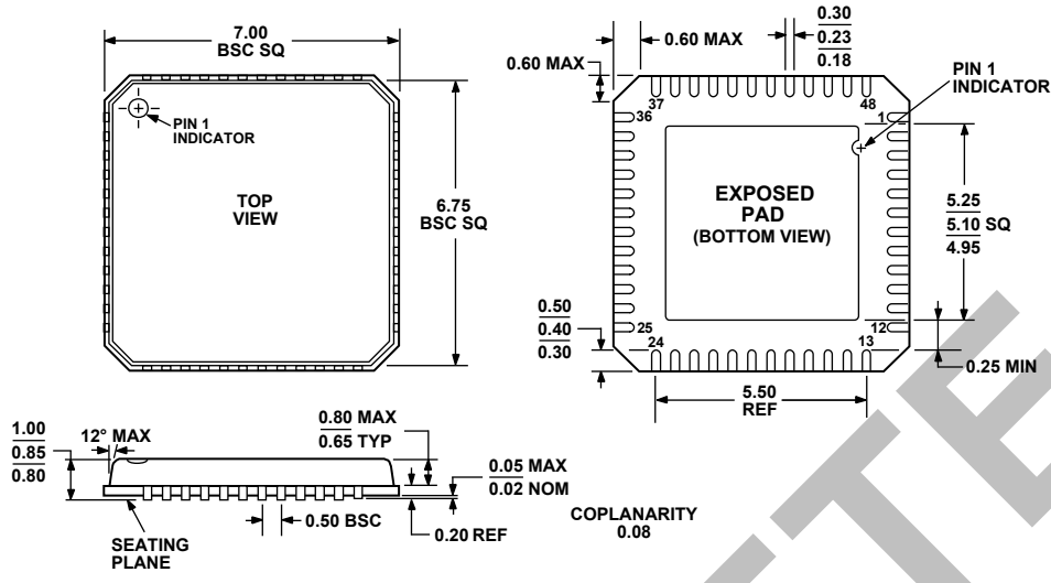
COMPLIANT TO JEDEC STANDARDS MO-220-VKGD-2 Figure 32. 48-Lead Lead Frame Chip Scale Package [LFCSP_VQ] 7 mm x 7 mm Body, Very Thin Quad (CP-48-1) Dimensions shown in millimeters
