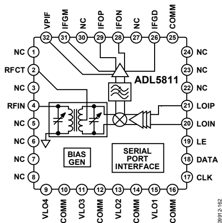
Figure 58. Block Diagram
