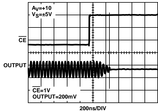
FIGURE 36. DISABLE RESPONSE/TURN-OFF TIME
