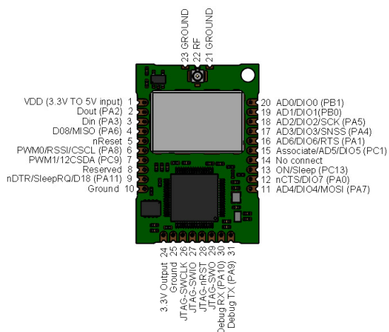
MTDOT-xxx-X1P-U.FL
